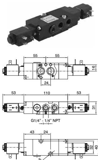
M51C.42.00.35.VC Peso 410 g
