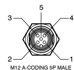
M12 A-CODING 5P MALE
