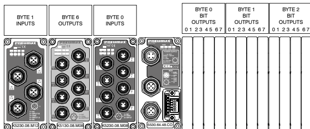
Example of input and output data distribution with CANopen interface 5530.64.48CO
