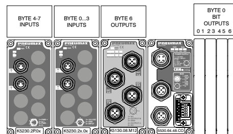
Example of input and output data distribution with CANopen interface 5530.64.48CO
