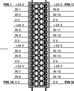
Morsetteria 32 pin
