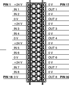
Morsetti a 32 pin
